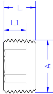
VIEW: B-B
