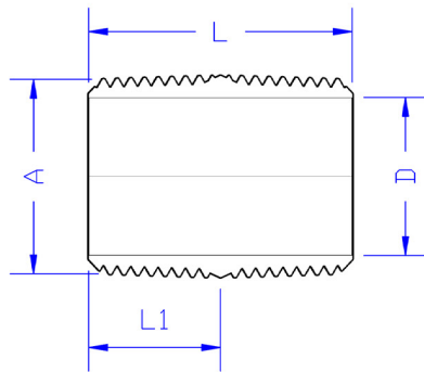
VIEW: B-B
