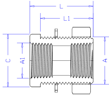
VIEW: B-B
